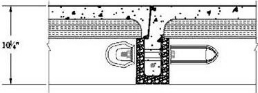
DETAIL B
