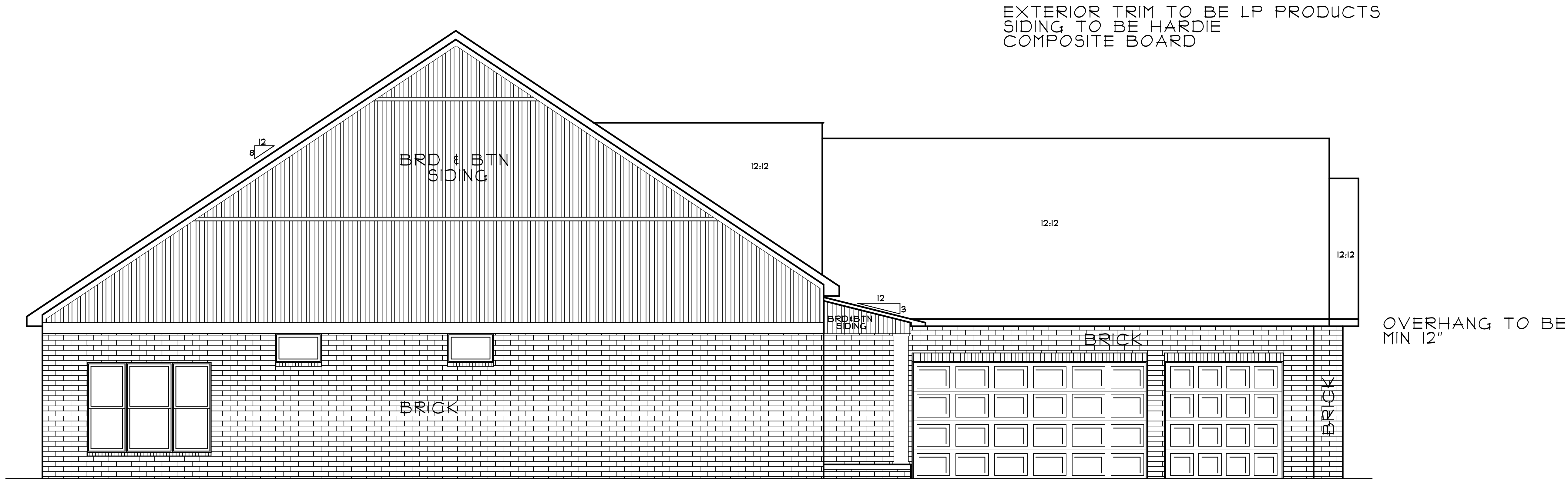
LEFT ELEVATION
